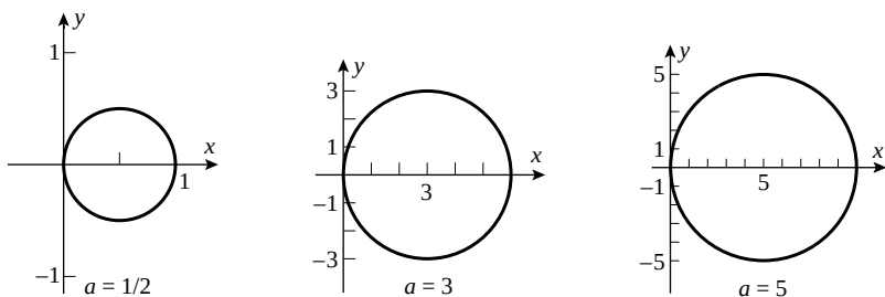
64. (a) a = 1/2
